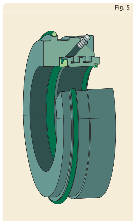
Taconite heavy-duty seal with a radial labyrinth
