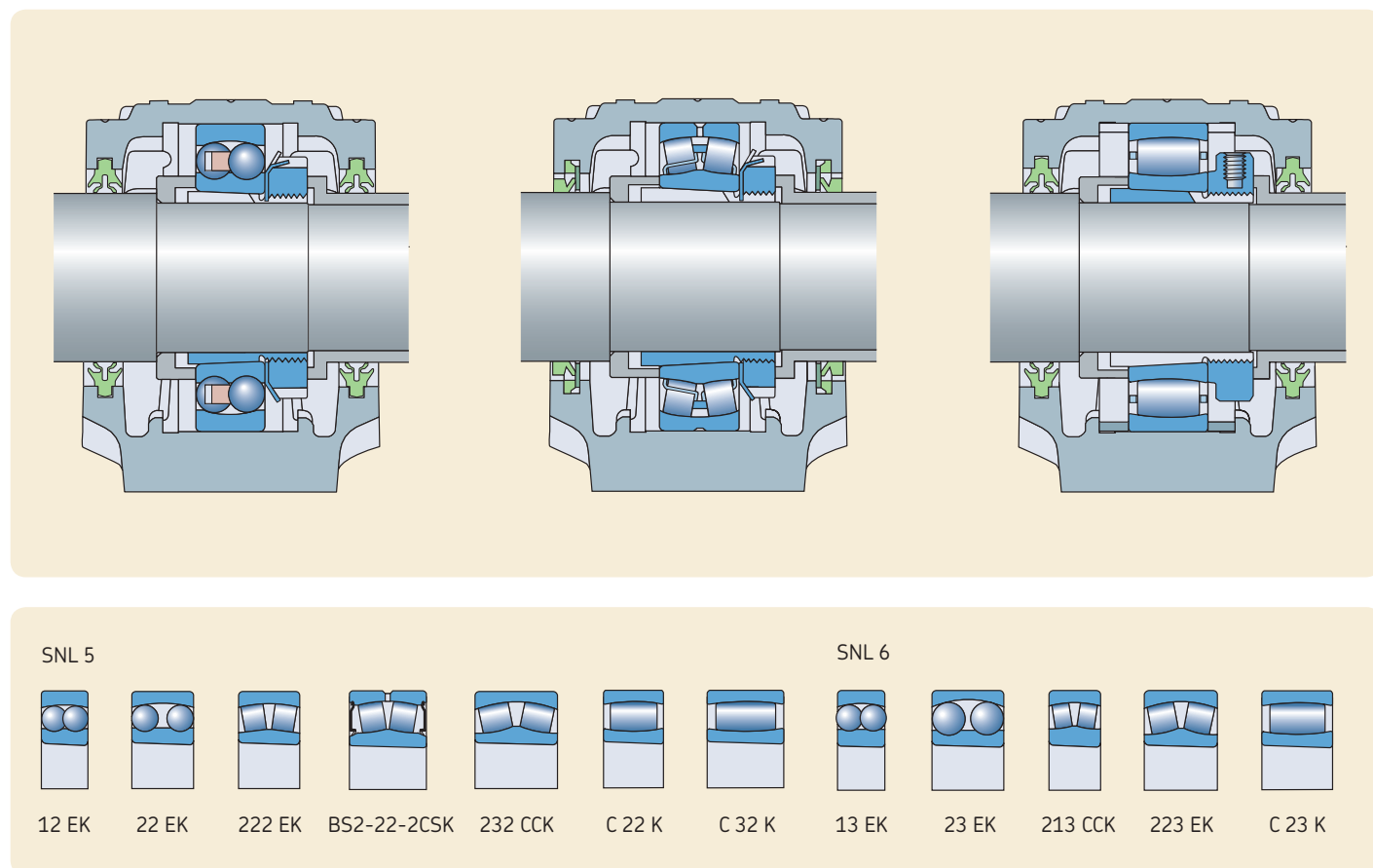
Bearings on adapter sleeves on stepped shafts
